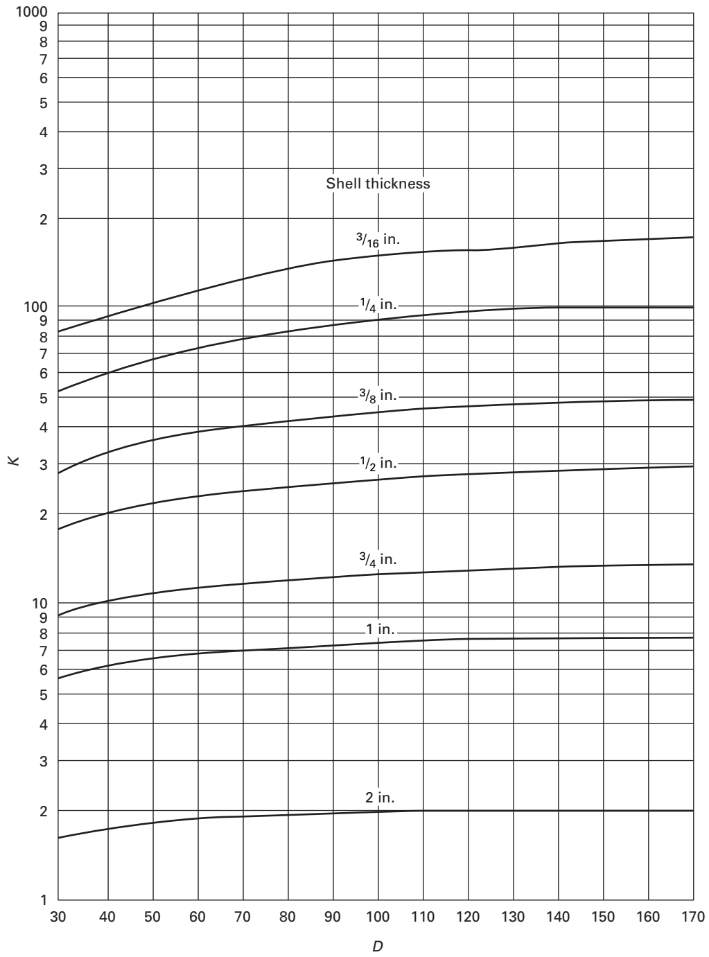
Figure EE-2 NPS 3 Pipe Jacket
