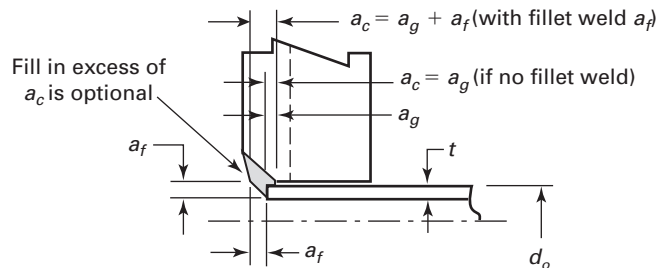
Combination Inset Fillet and Groove where: a_c = a_g + a_f and a_f \leq t (f)
