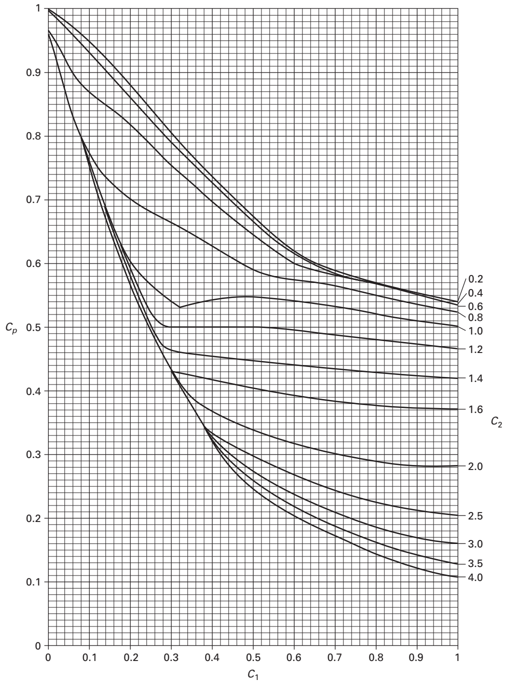
Figure 26-4 Coefficient C_p
