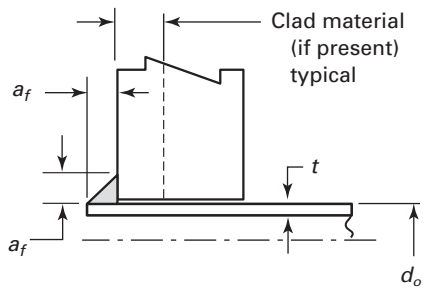
Face-Fillet Weld (a)
