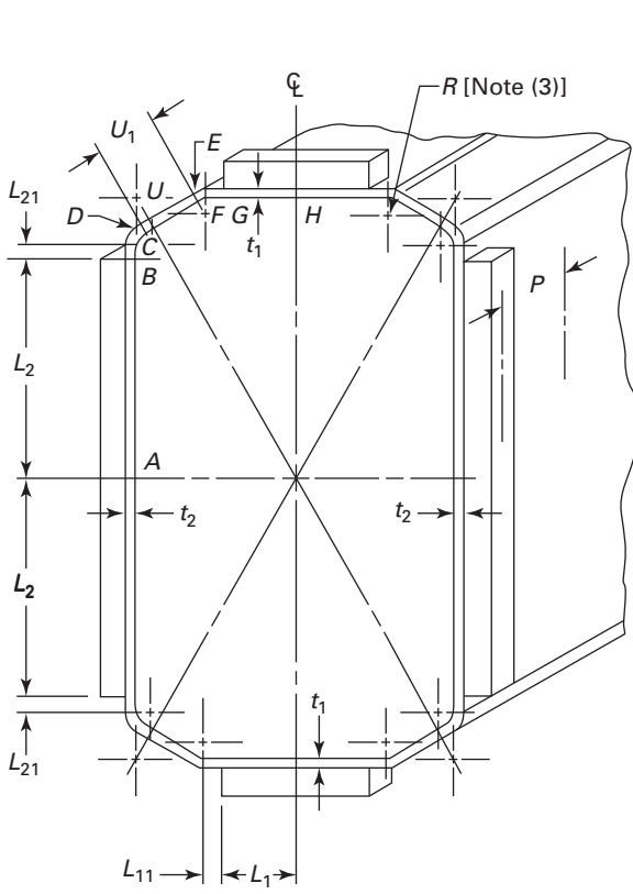
Figure 13-2(a) Vessels of Rectangular Cross Section (Cont'd)
