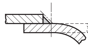
(h) Not Permissible
