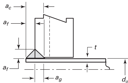
Combination Face-Fillet and Groove where: a_c = a_f + a_g and a_f = a_g (c)
