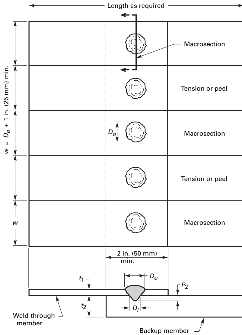
Figure 17-11 Gas Metal Arc-Spot-Weld Block for Macrosections and Strength Tests
