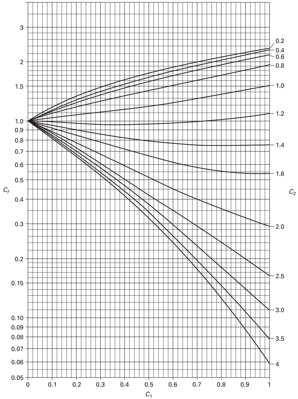
Figure 26-5 Coefficient C_f
