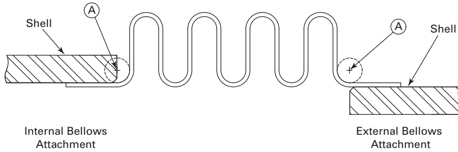
(a) U-Shaped Bellows
