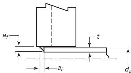
Inset Fillet Weld where: a_f \leq t (e)
