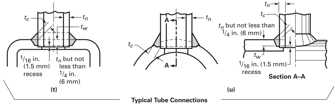
Typical Tube Connections
