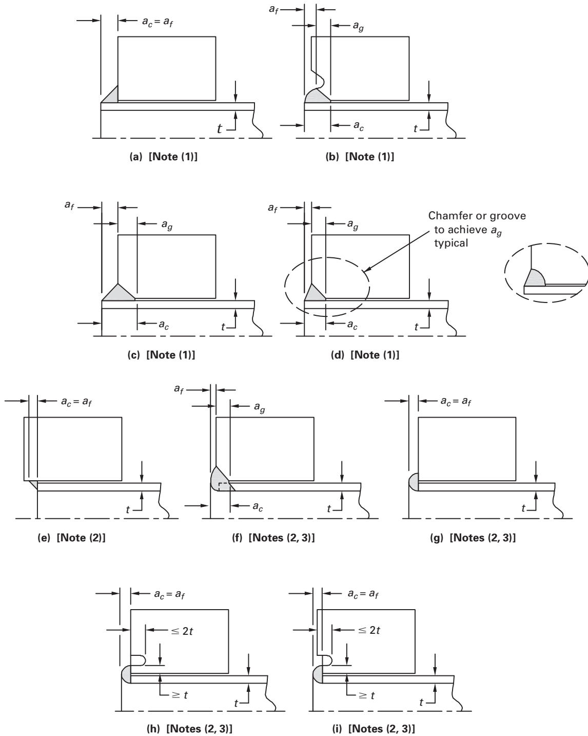
Figure A-2 Some Acceptable Types of Tube-to-Tubesheet Welds
