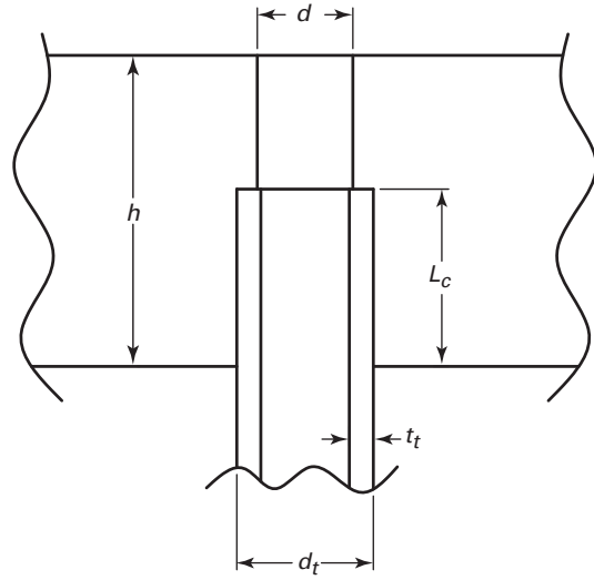
(b) Tube Joint
